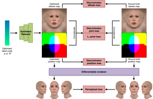
Figure 5: Our GAN-inversion searches a corresponding \mathbf{w} , which can reconstruct the target geometry and texture.
