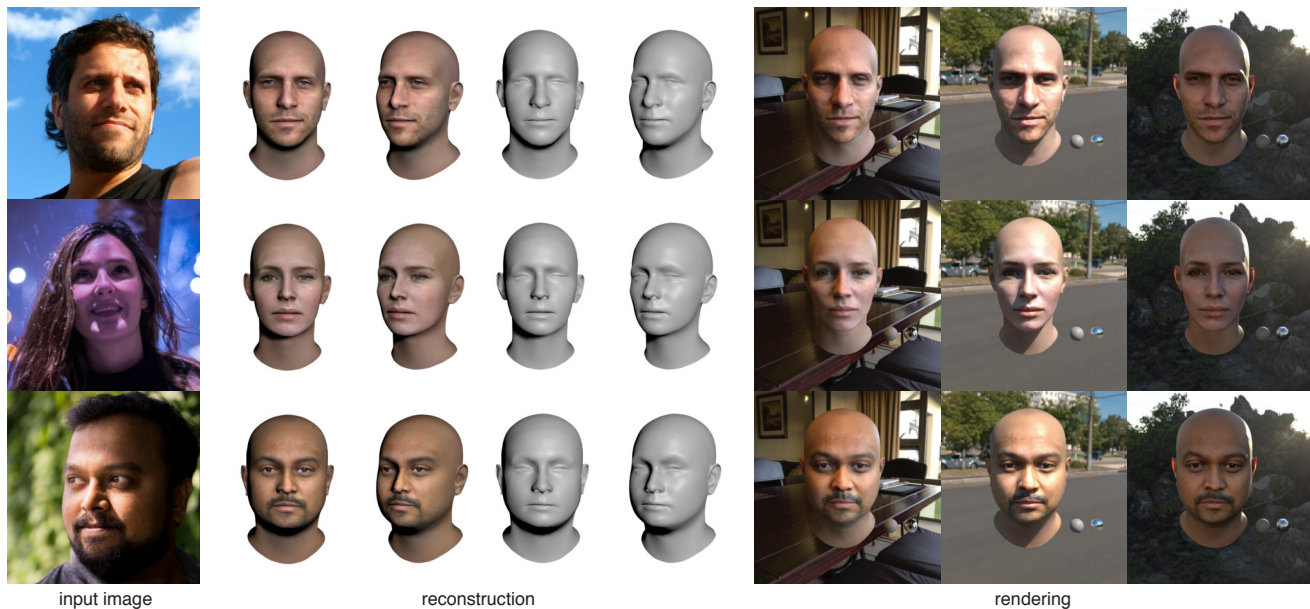
Figure 1: Given a single photograph, we can reconstruct a high-quality textured 3D face with neutral expression and normalized lighting condition. Our approach can handle extremely challenging cases and our generated avatars are animation friendly and suitable for complex relighting in virtual environments.
