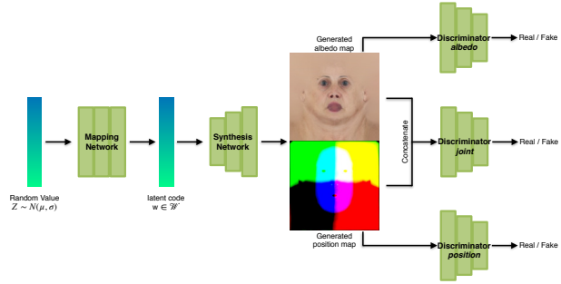
Figure 4: GAN-based geometry and texture synthesis.
