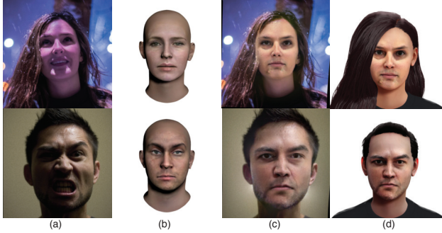
Figure 13: Qualitative comparison with state-of-the-art face normalization method [53]. From left to right, we show (a) input image; (b) our reconstructed result; (c) image-based face normalization result generated by Nagano et al. [53]; (d) Face2Face reconstruction result based on (c).
