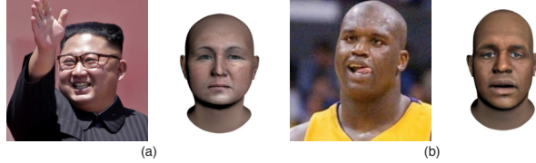
Figure 14: Failure cases in our experiments. (a) shows a failure where the specularity at the chin is baked into the generated result; (b) shows that the robustness of the reconstruction result is affected by the exaggerated expression.
