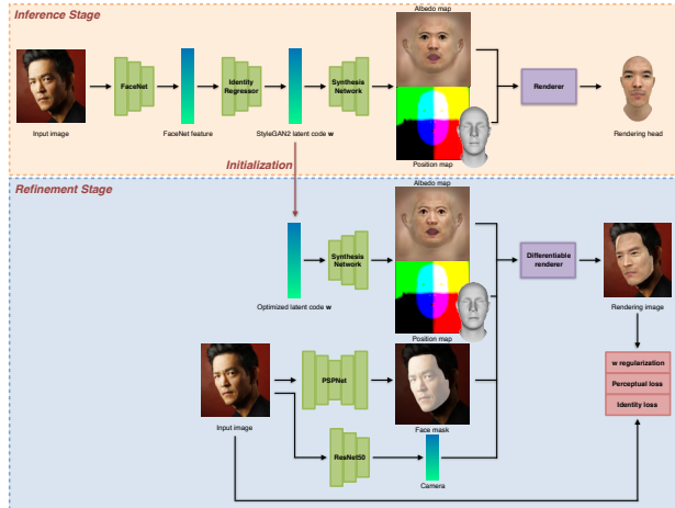
Figure 3: Two-stage facial digitization framework. The avatar is firstly predicted in the inference stage, and then improved to match the input image in the refinement stage.
