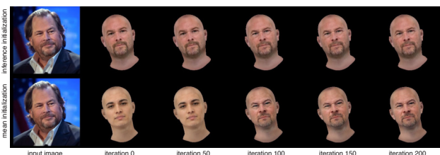
Figure 11: Qualitative comparison with different initialization schemes for iterative refinement. The mean initialization starts optimization from a mean latent vector of our training dataset. The inference initialization starts from the latent vector predicted by R .
